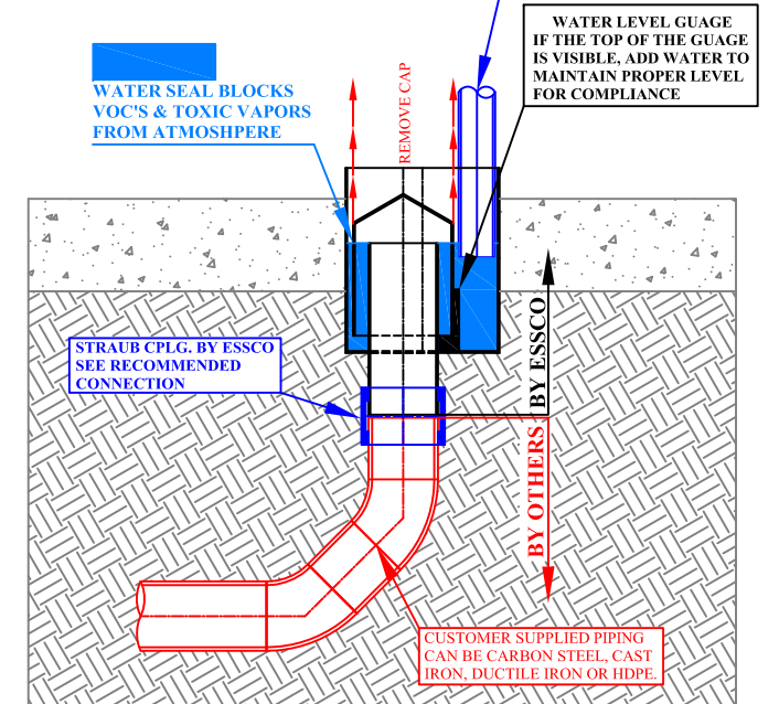
ESSCO DRAIN HUB FOR PUMP OR VESSEL DRAINS QQQ, B-1, HON & NSPS COMPLIANT INSTALLATION
