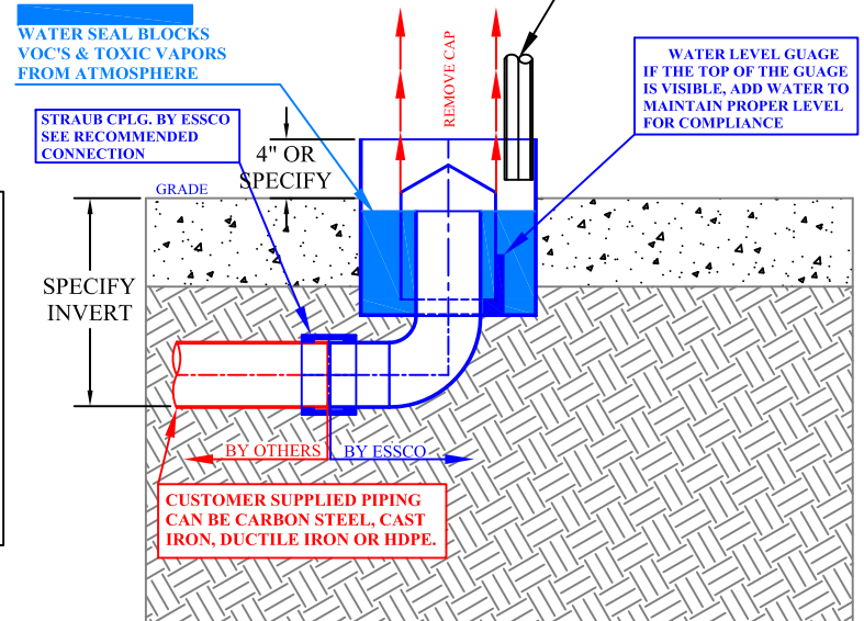
ESSCO DRAIN HUB FOR QQQ, B-1, HON & NSPS COMPLIANT PUMP OR VESSEL INSTALLATION
